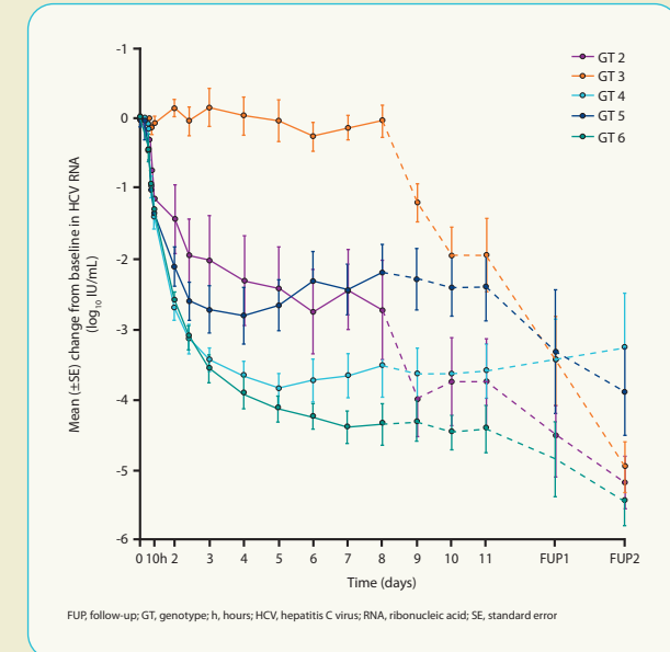
Figure 3. Mean (±SE) change from baseline in plasma HCV RNA (log 10 IU/mL) for each GT cohort.
